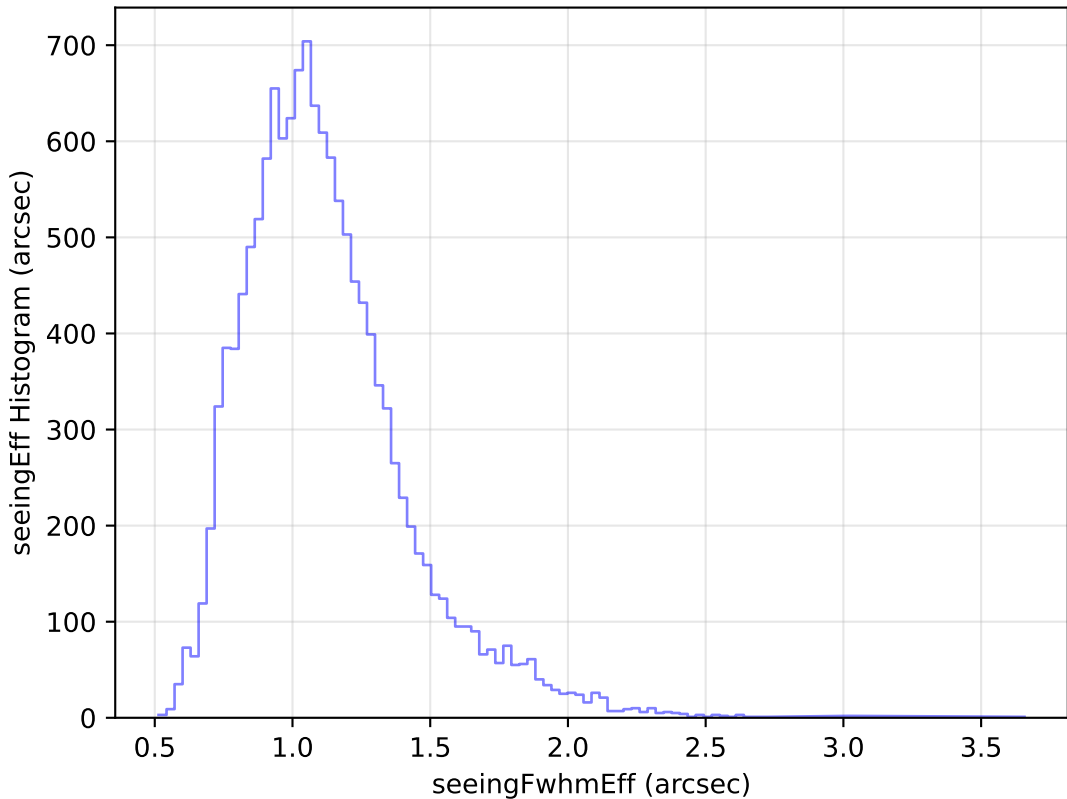
baseline_v2.0_10yrs Yr 1 u band: seeingEff Histogram
