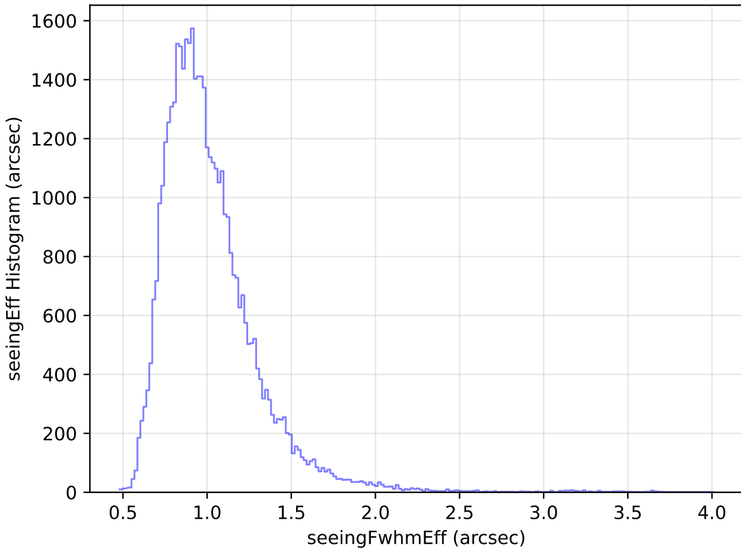
baseline_v2.0_10yrs Yr 1 r band: seeingEff Histogram
