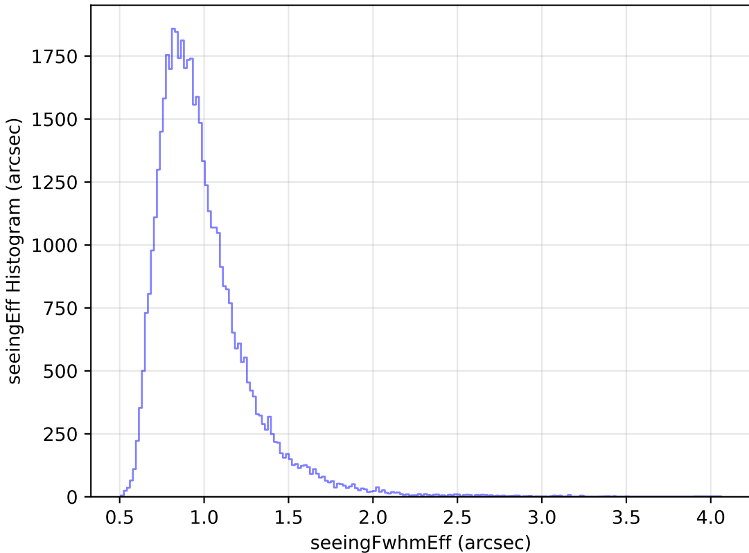
baseline_v2.0_10yrs Yr 1 i band: seeingEff Histogram
