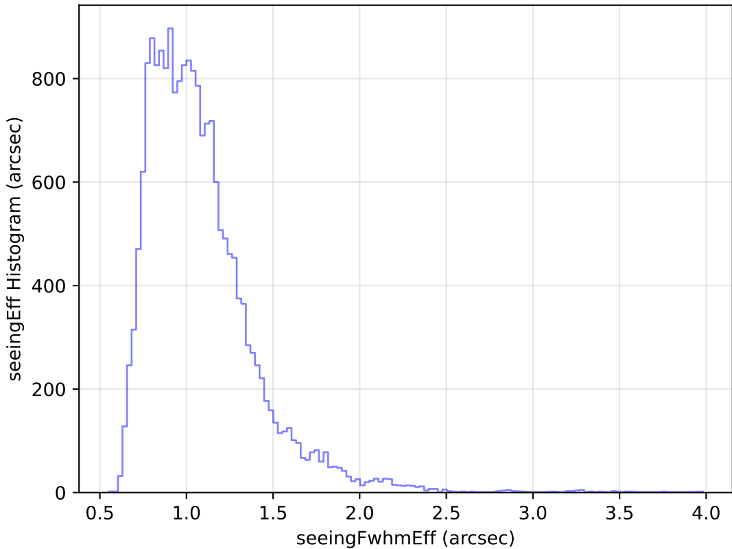
baseline_v2.0_10yrs Yr 1 g band: seeingEff Histogram
