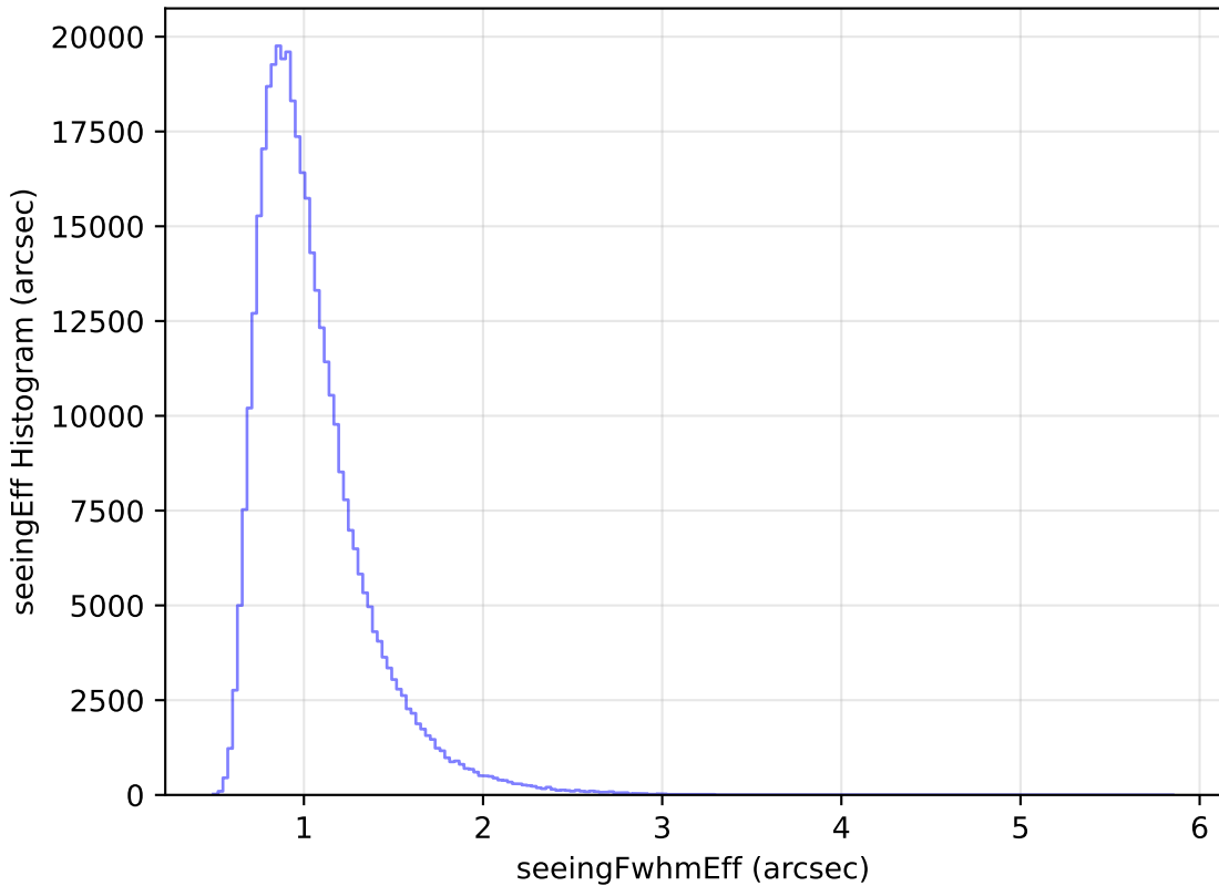
baseline_v2.0_10yrs WFD z band: seeingEff Histogram
