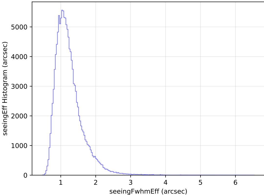
baseline_v2.0_10yrs WFD u band: seeingEff Histogram
