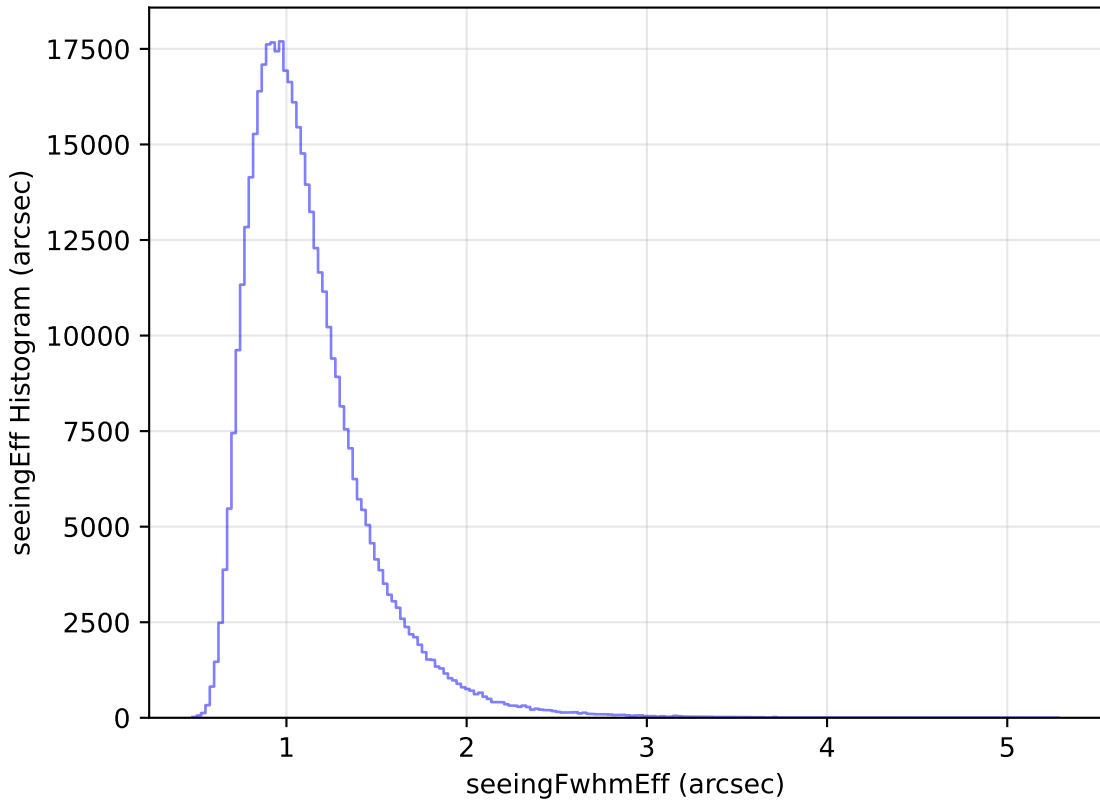
baseline_v2.0_10yrs WFD r band: seeingEff Histogram
