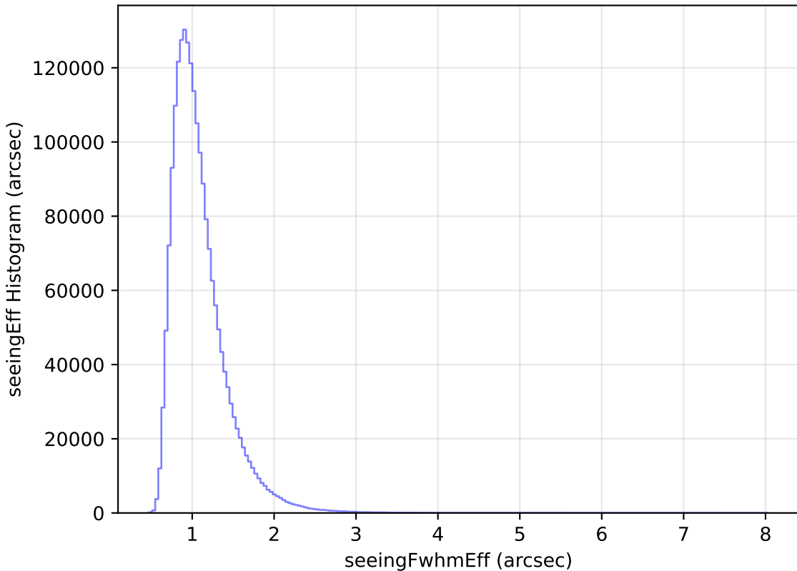
baseline_v2.0_10yrs WFD all bands: seeingEff Histogram
