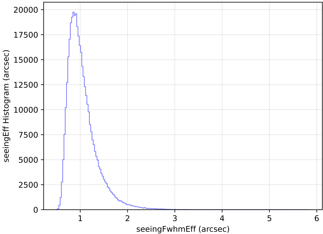
baseline_v2.0_10yrs All sky z band: seeingEff Histogram
