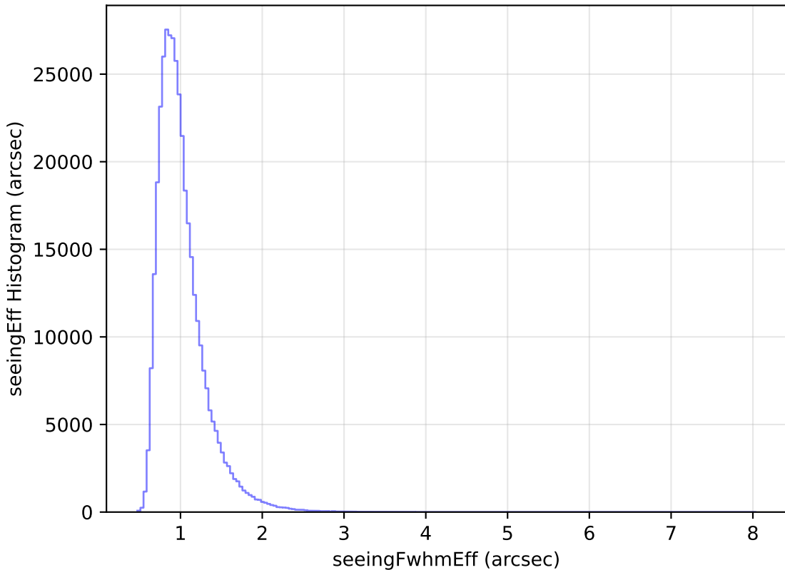
baseline_v2.0_10yrs All sky y band: seeingEff Histogram
