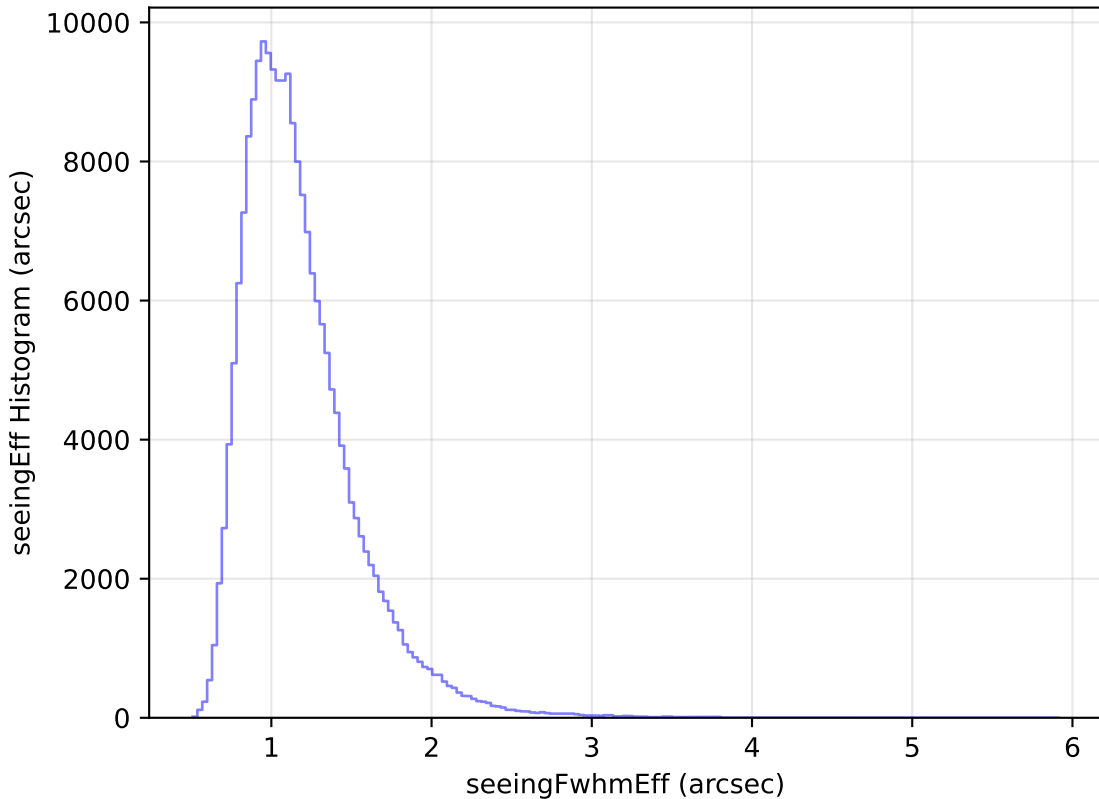
baseline_v2.0_10yrs All sky g band: seeingEff Histogram
