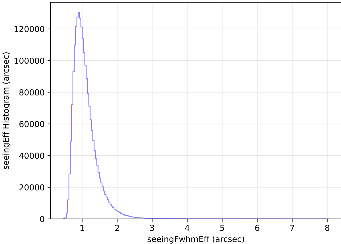
baseline_v2.0_10yrs All sky all bands: seeingEff Histogram
