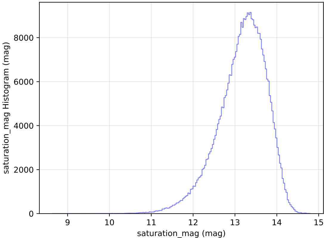
baseline_v2.0_10yrs WFD y band: saturation_mag Histogram
