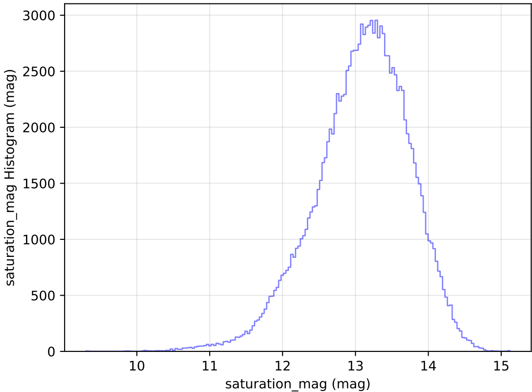
baseline_v2.0_10yrs WFD u band: saturation_mag Histogram
