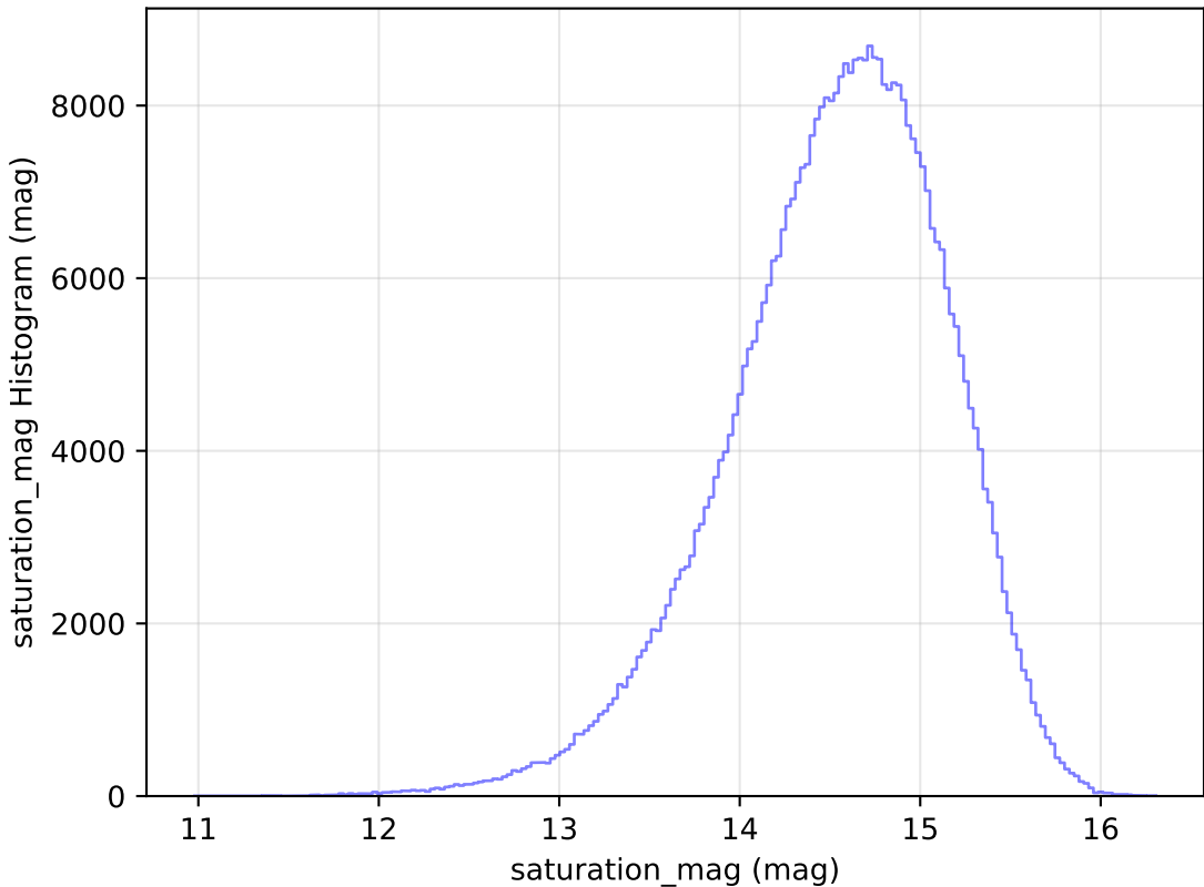
baseline_v2.0_10yrs WFD r band: saturation_mag Histogram
