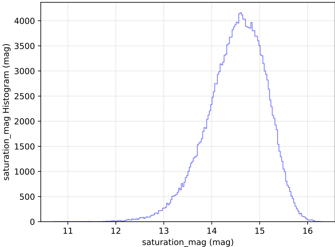
baseline_v2.0_10yrs WFD g band: saturation_mag Histogram
