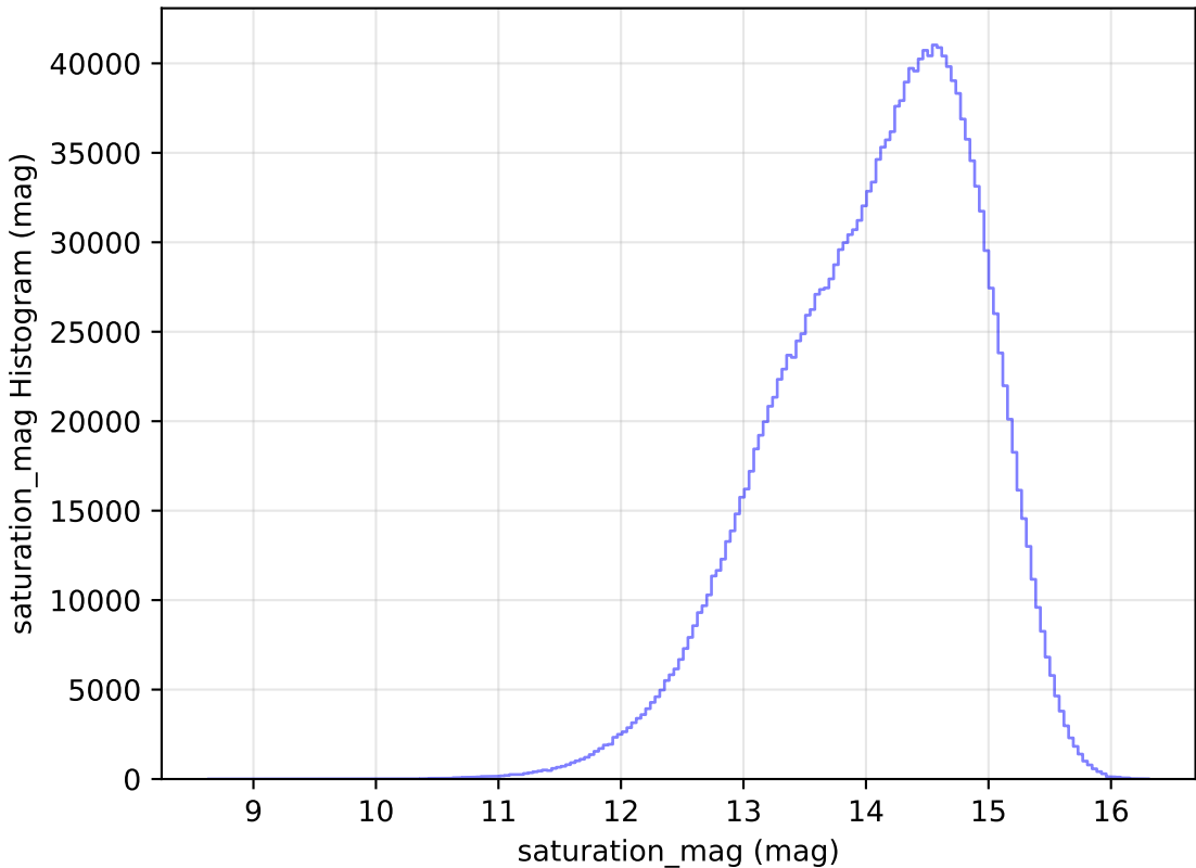
baseline_v2.0_10yrs WFD all bands: saturation_mag Histogram
