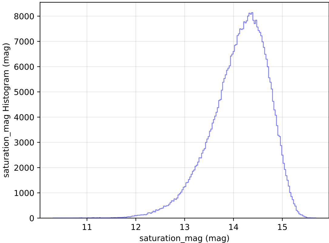
baseline_v2.0_10yrs All sky z band: saturation_mag Histogram
