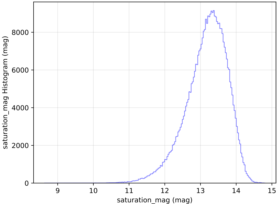
baseline_v2.0_10yrs All sky y band: saturation_mag Histogram
