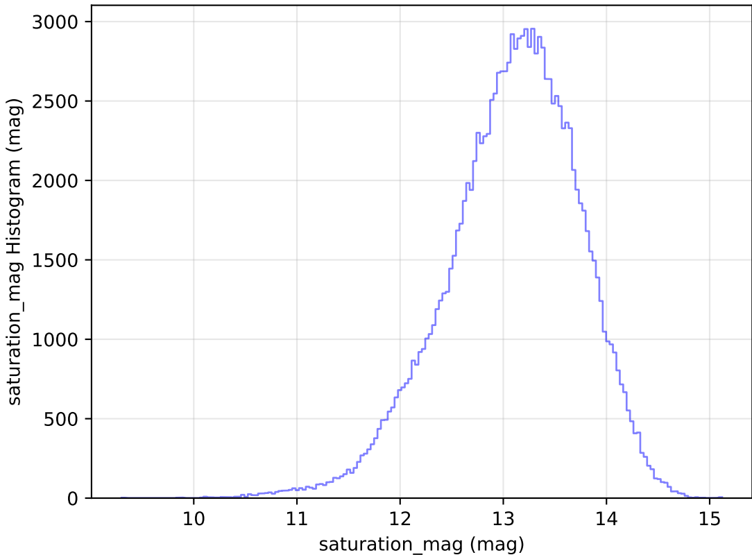
baseline_v2.0_10yrs All sky u band: saturation_mag Histogram
