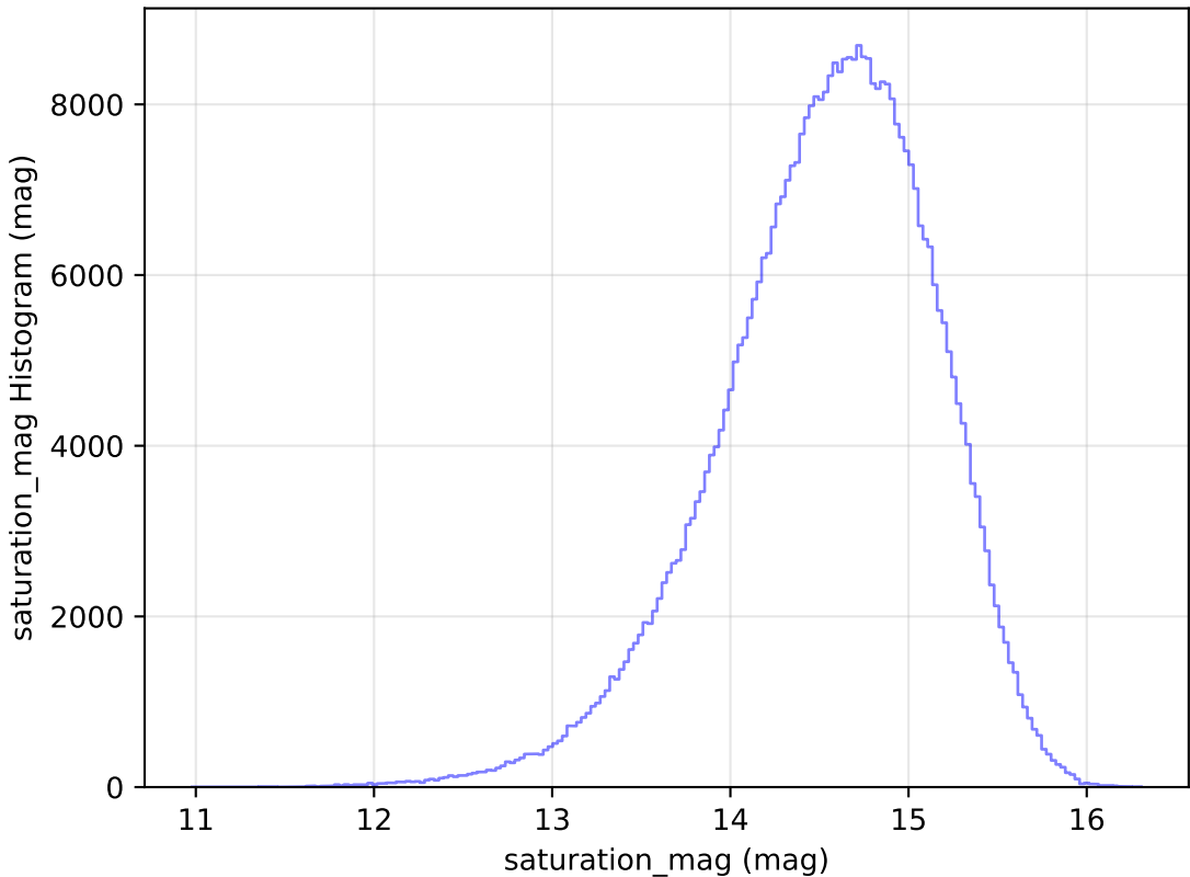
baseline_v2.0_10yrs All sky r band: saturation_mag Histogram
