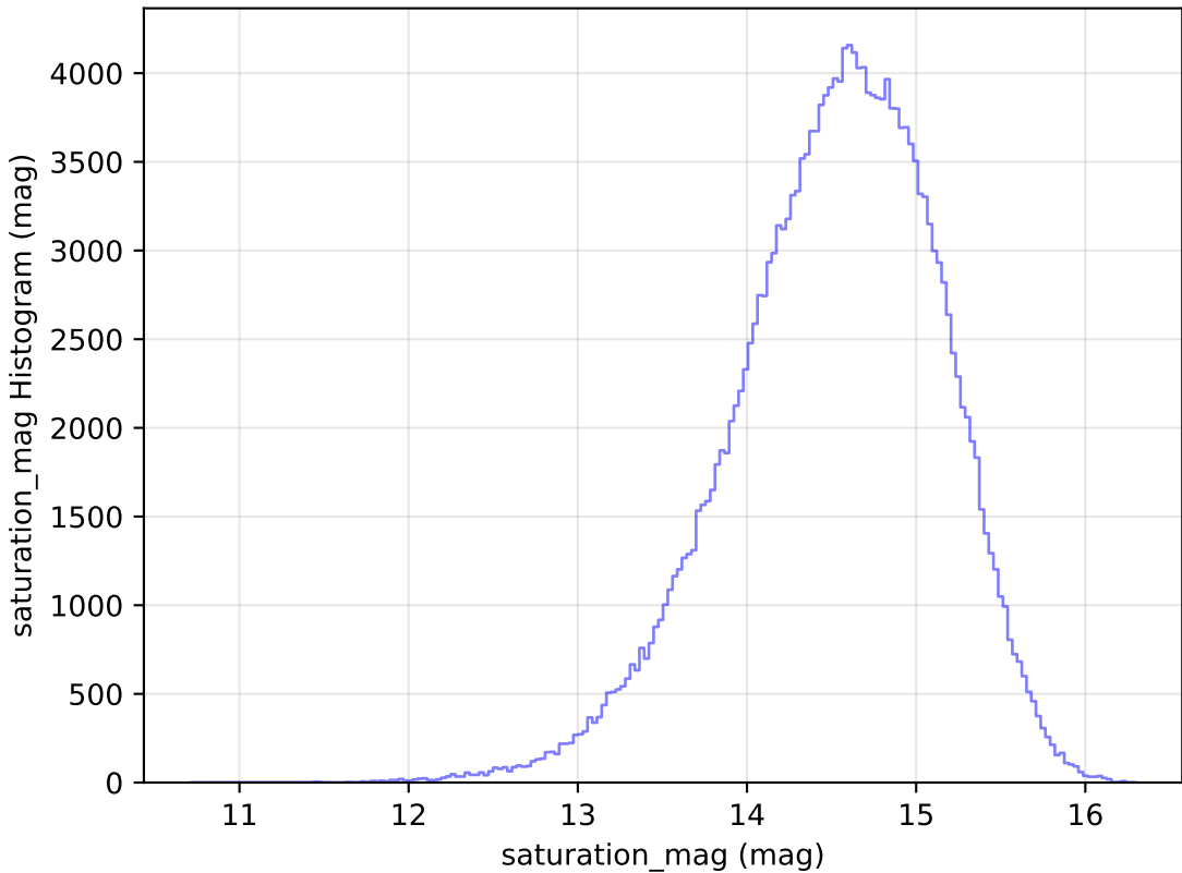
baseline_v2.0_10yrs All sky g band: saturation_mag Histogram
