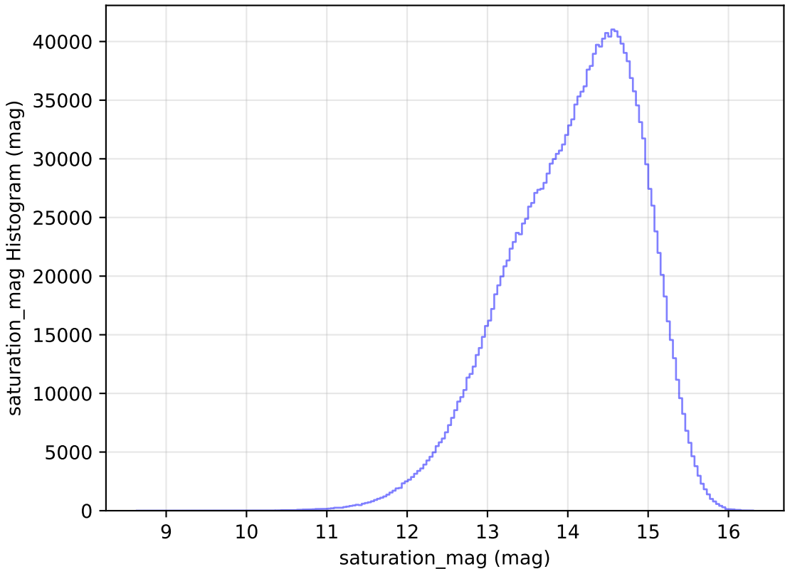
baseline_v2.0_10yrs All sky all bands: saturation_mag Histogram
