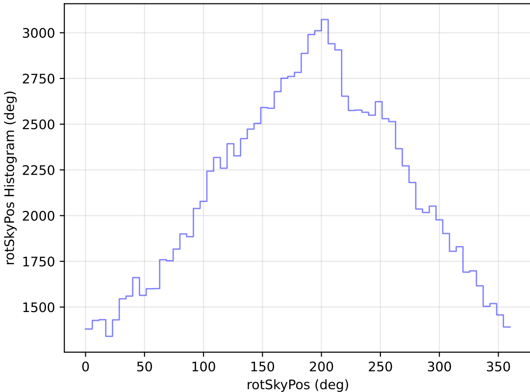
baseline_v2.0_10yrs WFD u band: rotSkyPos Histogram
