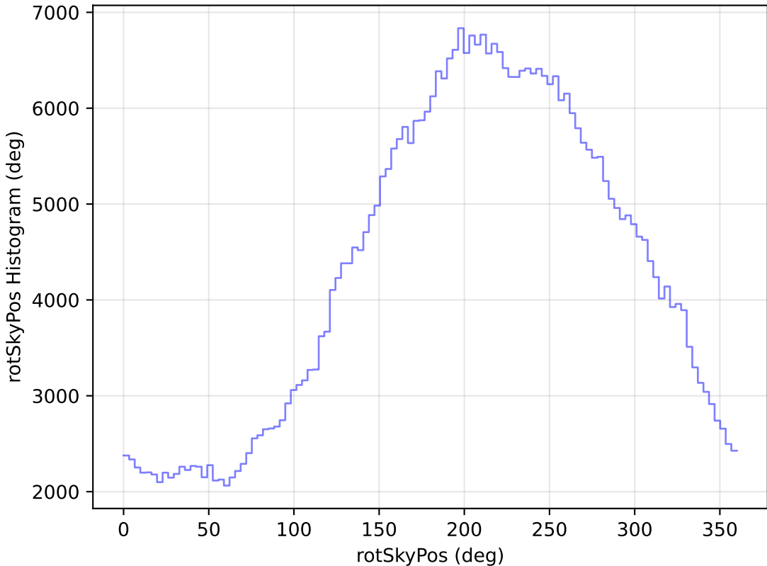
baseline_v2.0_10yrs WFD i band: rotSkyPos Histogram
