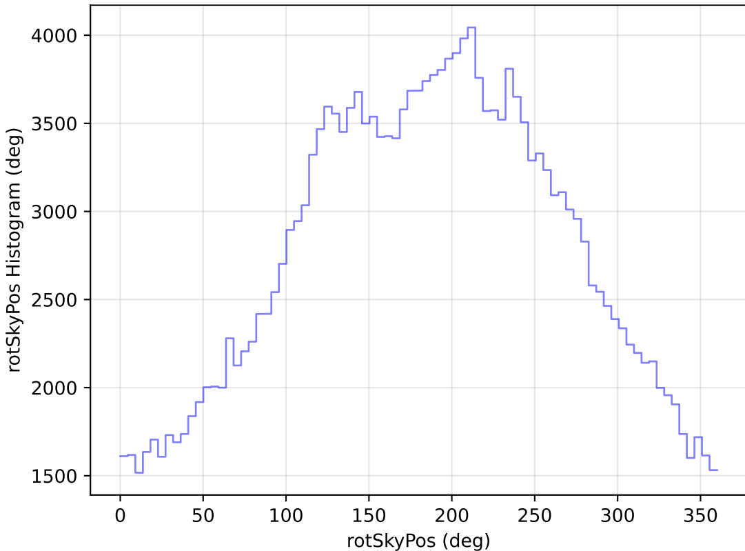
baseline_v2.0_10yrs WFD g band: rotSkyPos Histogram
