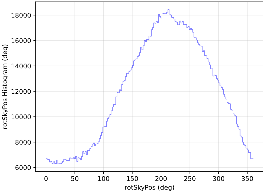
baseline_v2.0_10yrs WFD all bands: rotSkyPos Histogram
