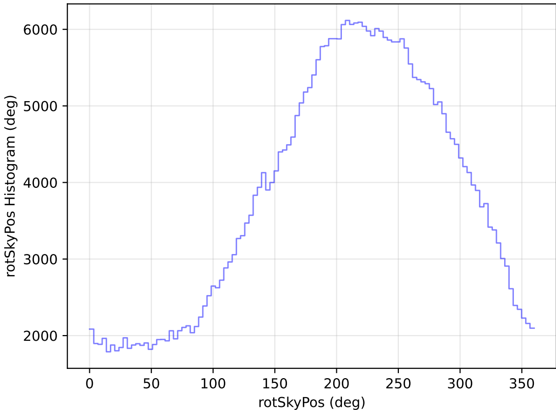
baseline_v2.0_10yrs All sky z band: rotSkyPos Histogram
