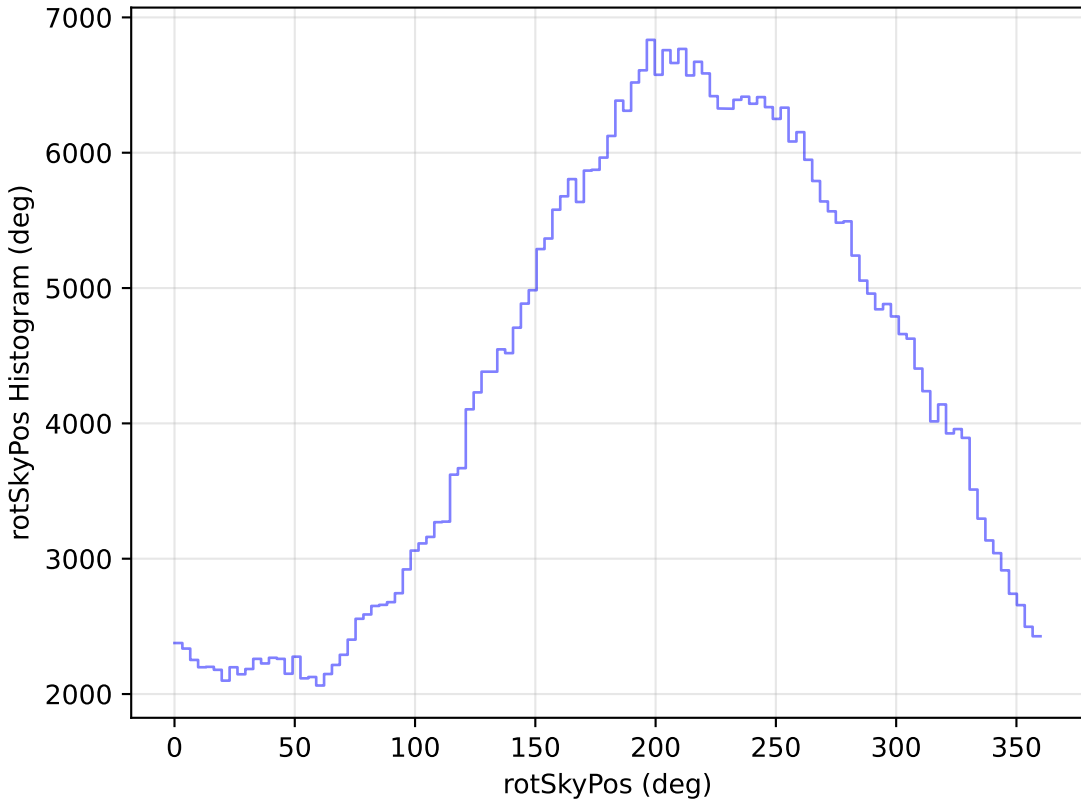
baseline_v2.0_10yrs All sky i band: rotSkyPos Histogram
