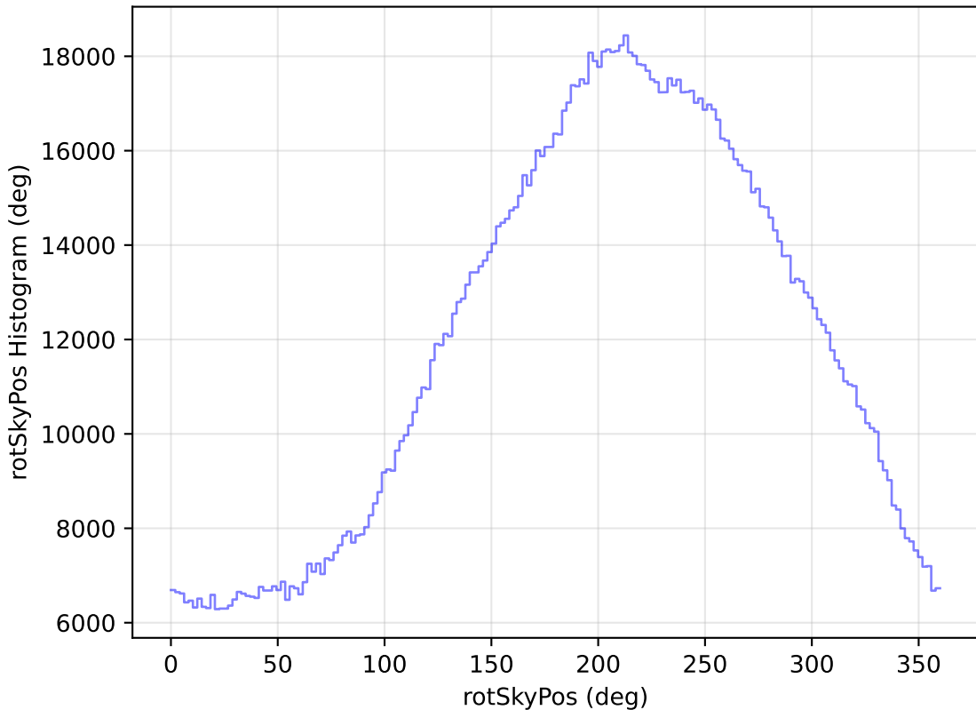
baseline_v2.0_10yrs All sky all bands: rotSkyPos Histogram
