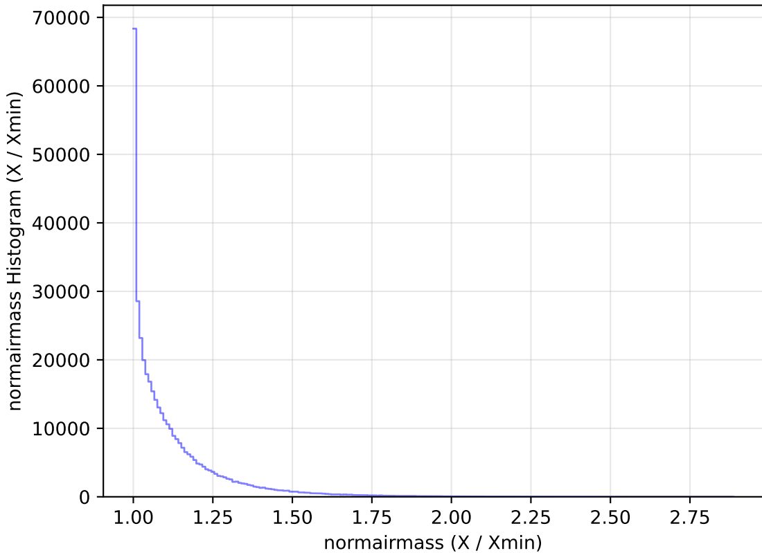
baseline_v2.0_10yrs WFD z band: normairmass Histogram
