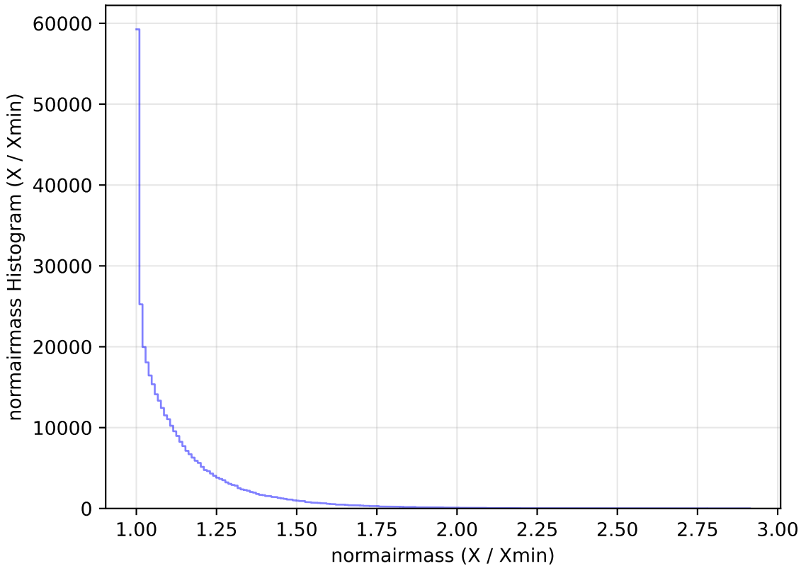
baseline_v2.0_10yrs WFD y band: normairmass Histogram
