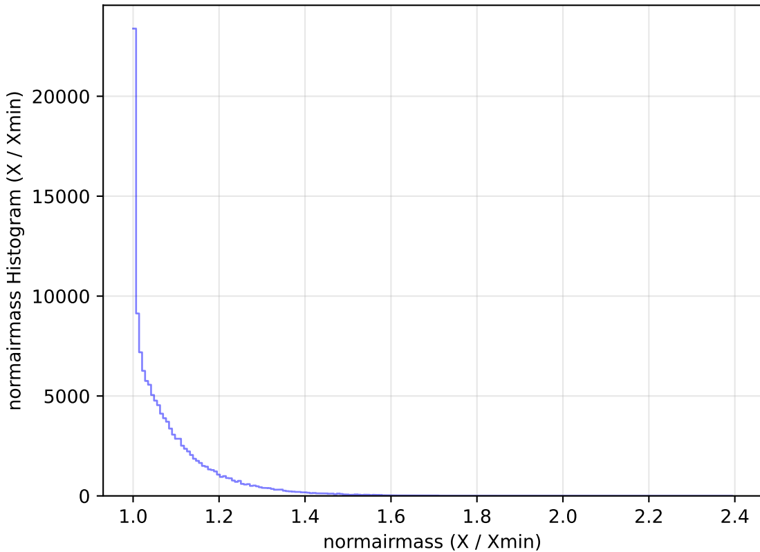
baseline_v2.0_10yrs WFD u band: normairmass Histogram
