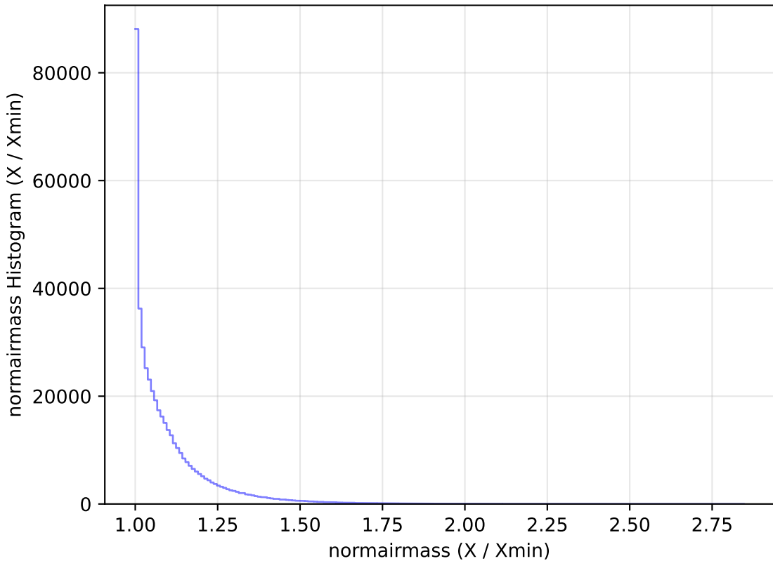
baseline_v2.0_10yrs WFD r band: normairmass Histogram
