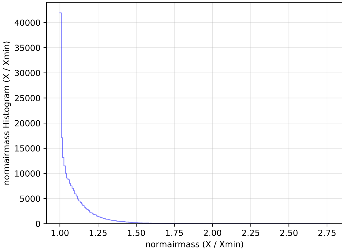
baseline_v2.0_10yrs WFD g band: normairmass Histogram
