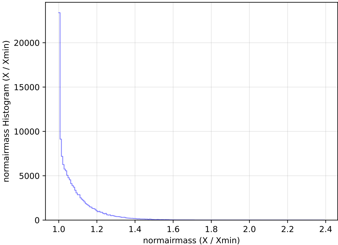
baseline_v2.0_10yrs All sky u band: normairmass Histogram
