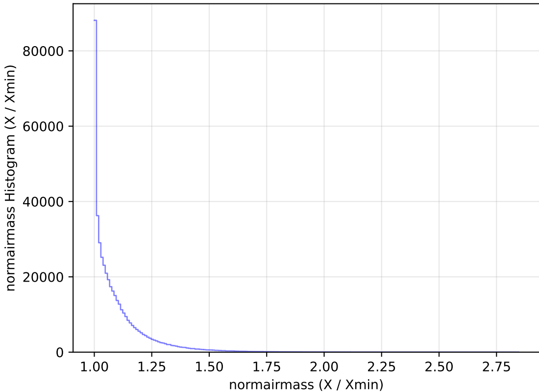
baseline_v2.0_10yrs All sky r band: normairmass Histogram
