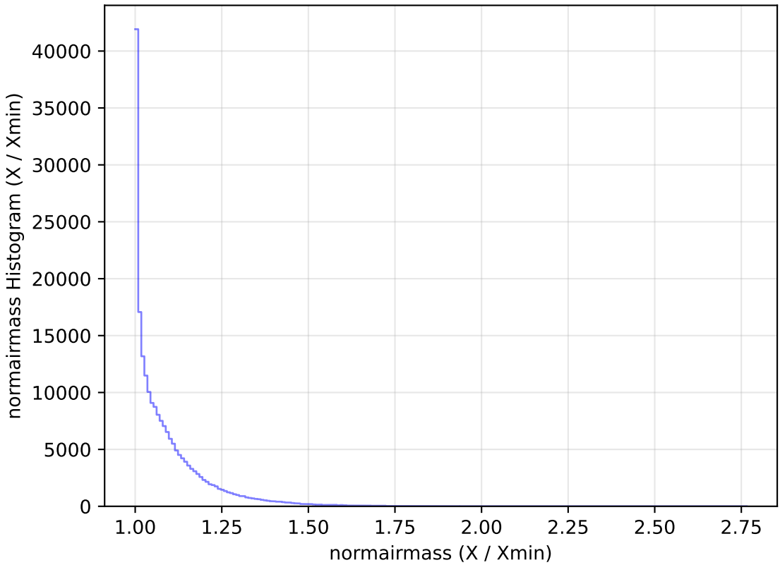
baseline_v2.0_10yrs All sky g band: normairmass Histogram
