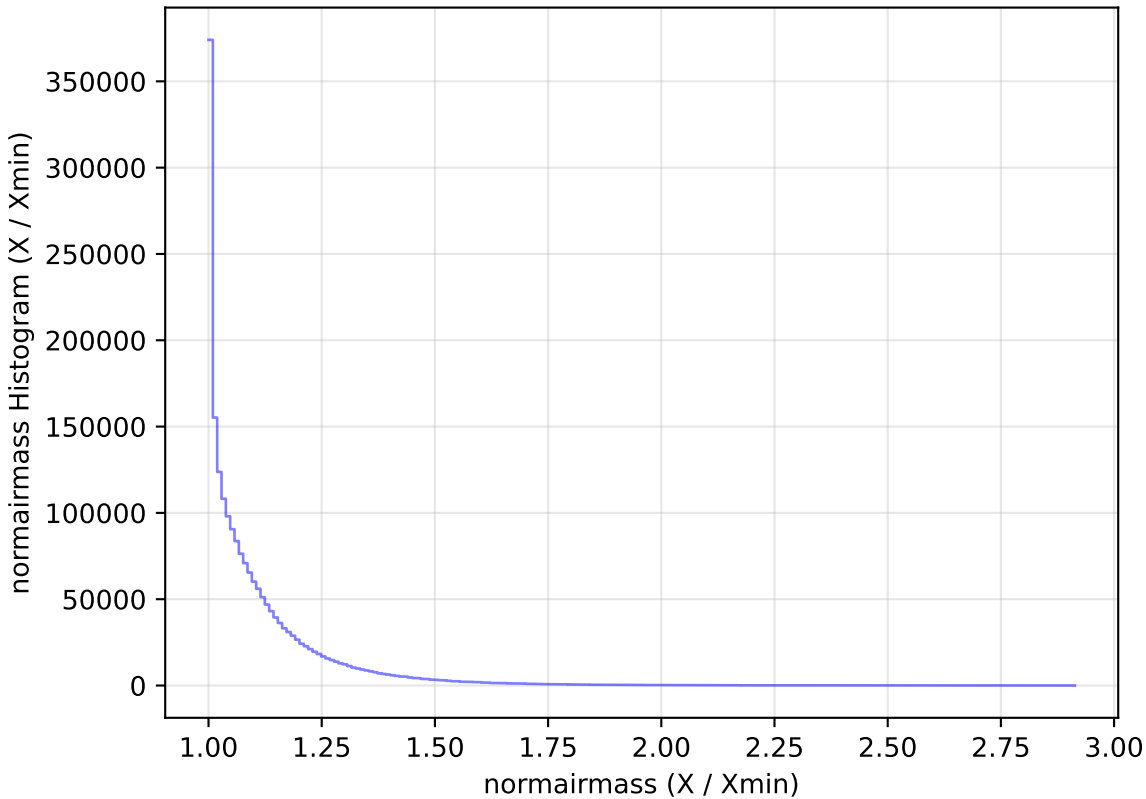
baseline_v2.0_10yrs All sky all bands: normairmass Histogram
