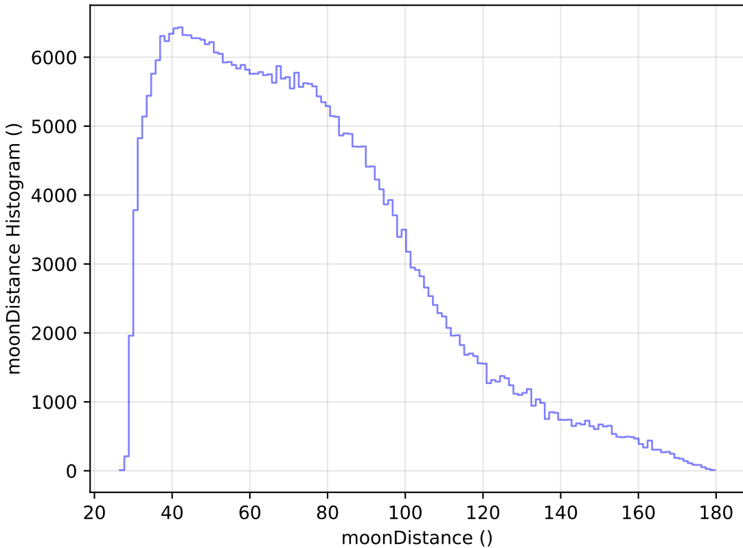
baseline_v2.0_10yrs WFD z band: moonDistance Histogram
