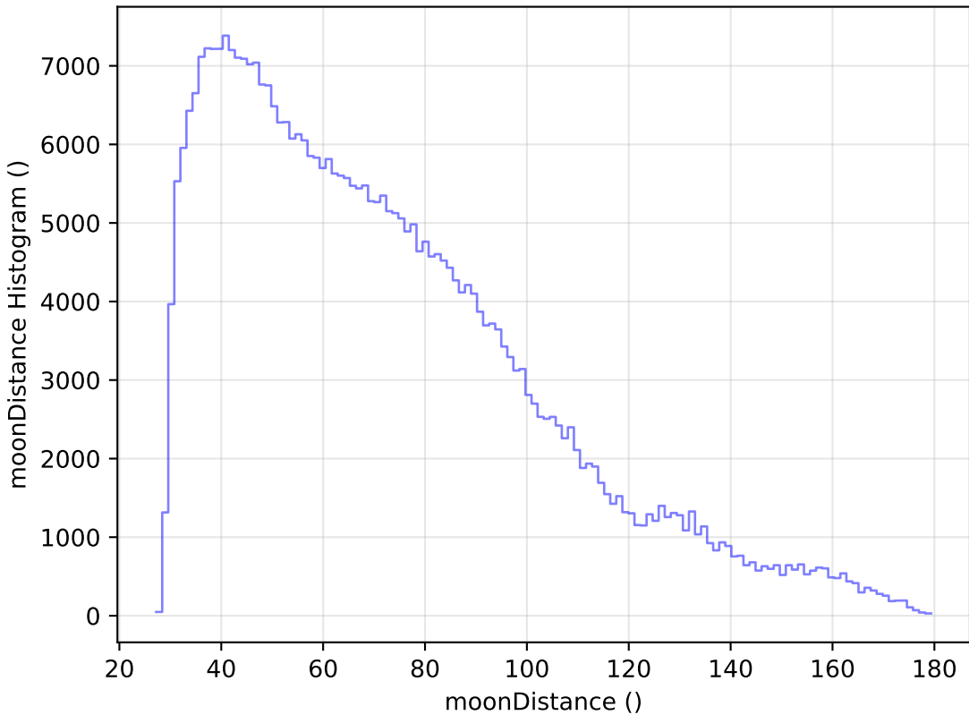
baseline_v2.0_10yrs WFD y band: moonDistance Histogram
