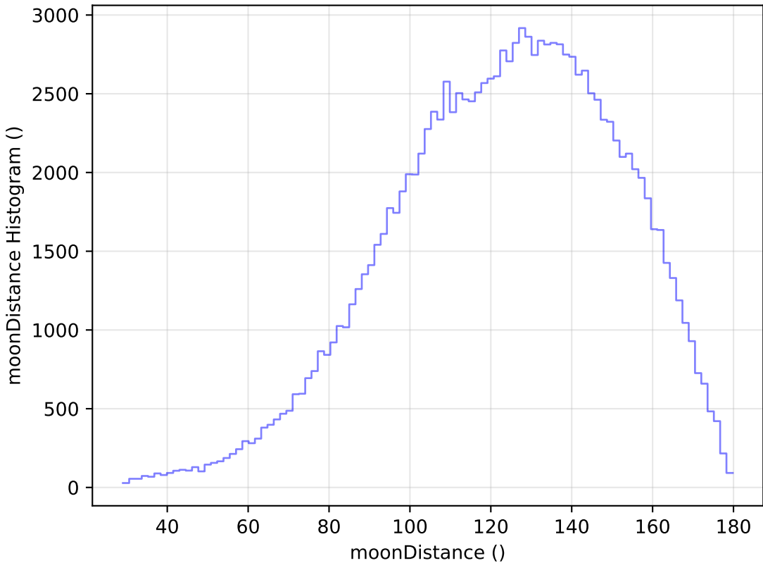
baseline_v2.0_10yrs WFD u band: moonDistance Histogram
