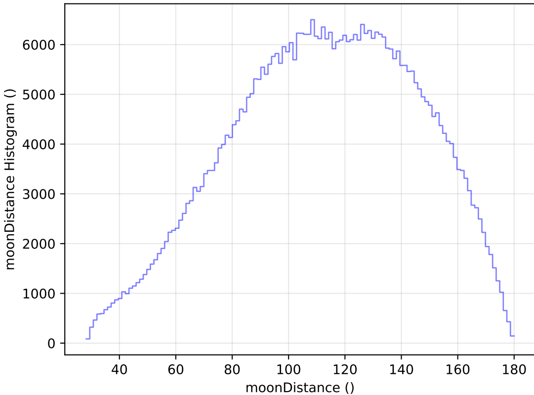
baseline_v2.0_10yrs WFD r band: moonDistance Histogram
