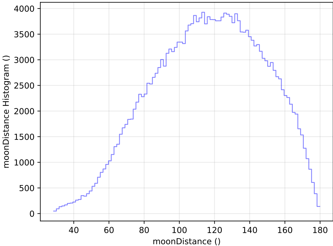
baseline_v2.0_10yrs WFD g band: moonDistance Histogram
