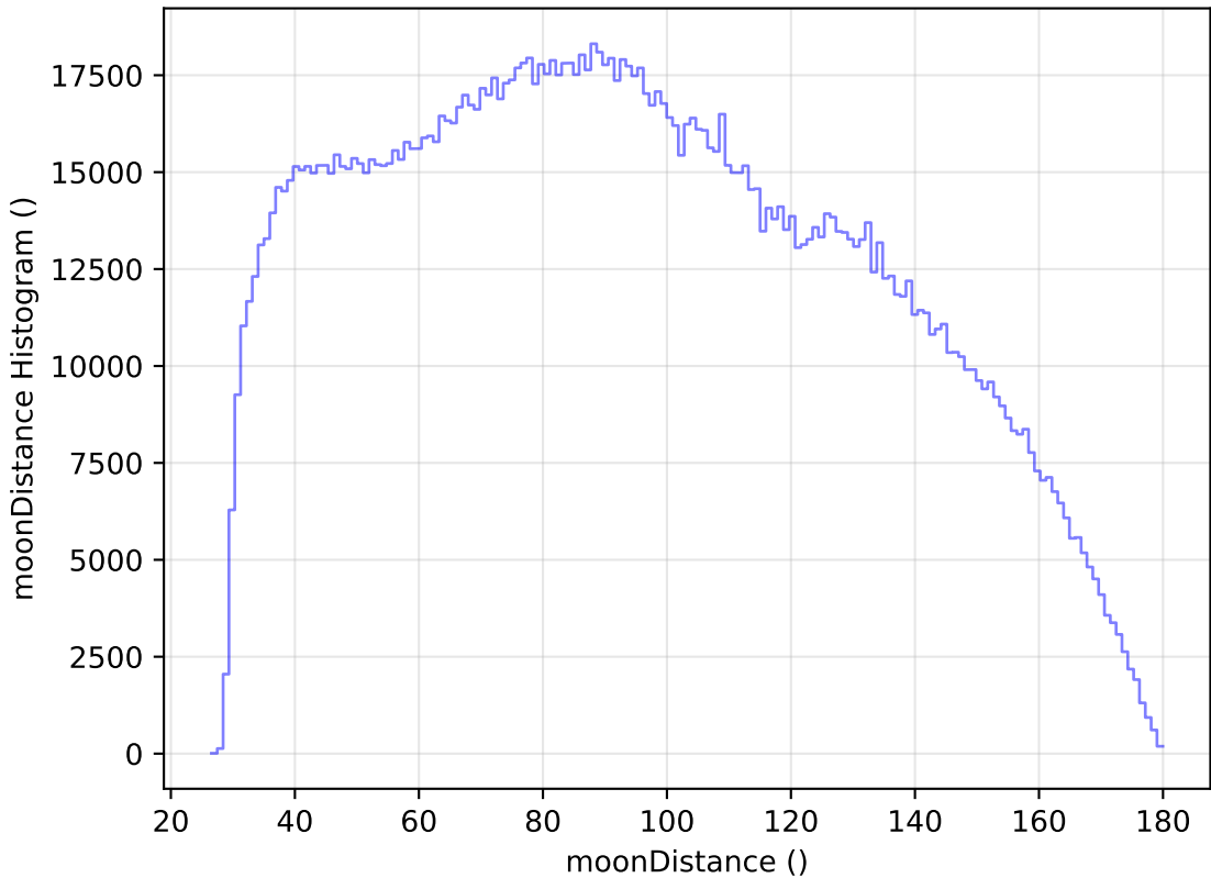
baseline_v2.0_10yrs WFD all bands: moonDistance Histogram
