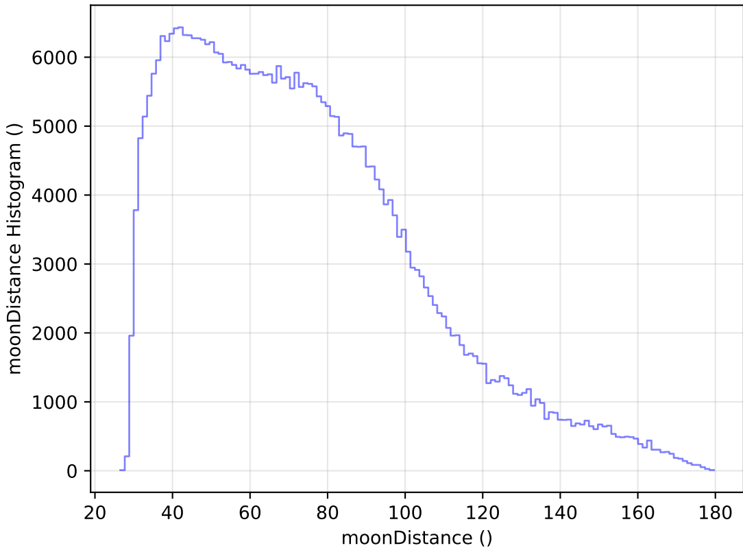
baseline_v2.0_10yrs All sky z band: moonDistance Histogram
