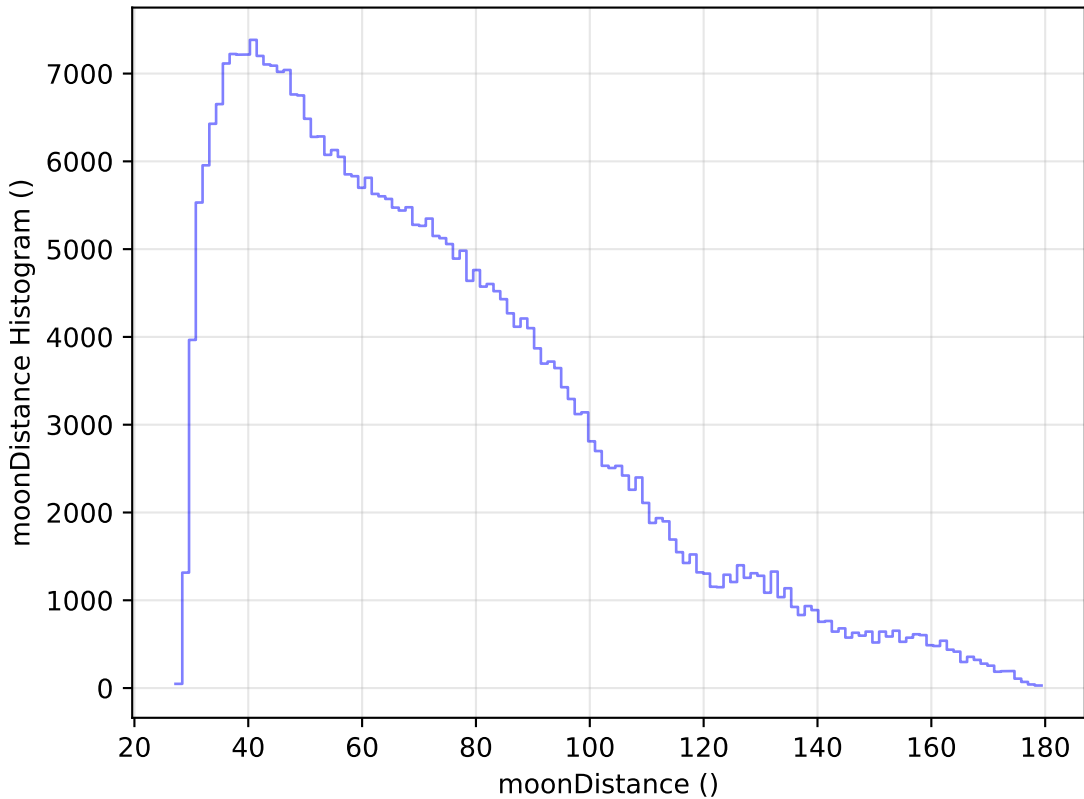
baseline_v2.0_10yrs All sky y band: moonDistance Histogram
