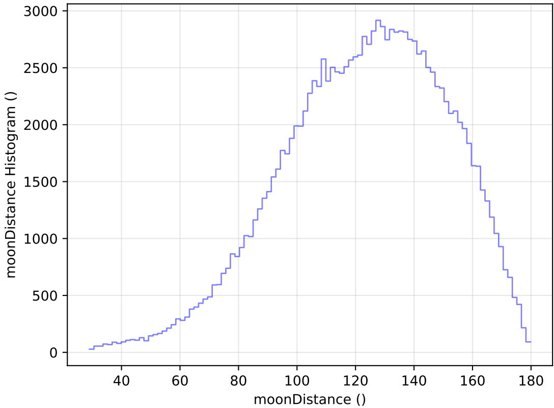
baseline_v2.0_10yrs All sky u band: moonDistance Histogram
