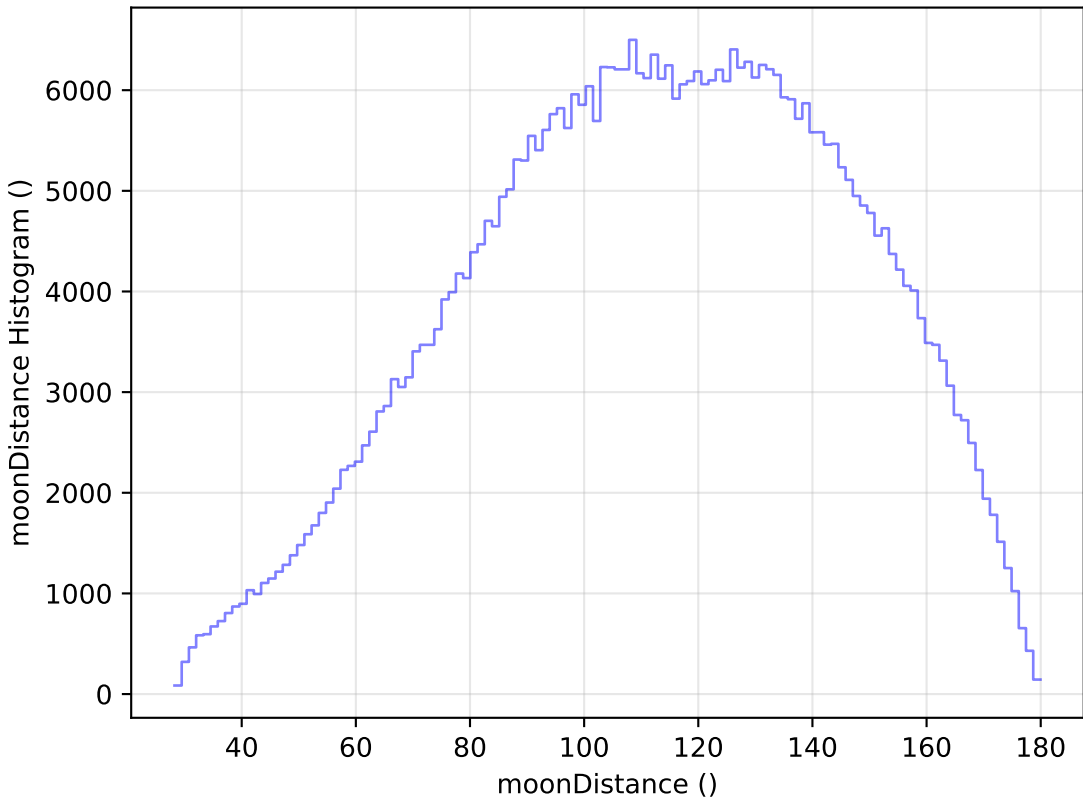
baseline_v2.0_10yrs All sky r band: moonDistance Histogram
