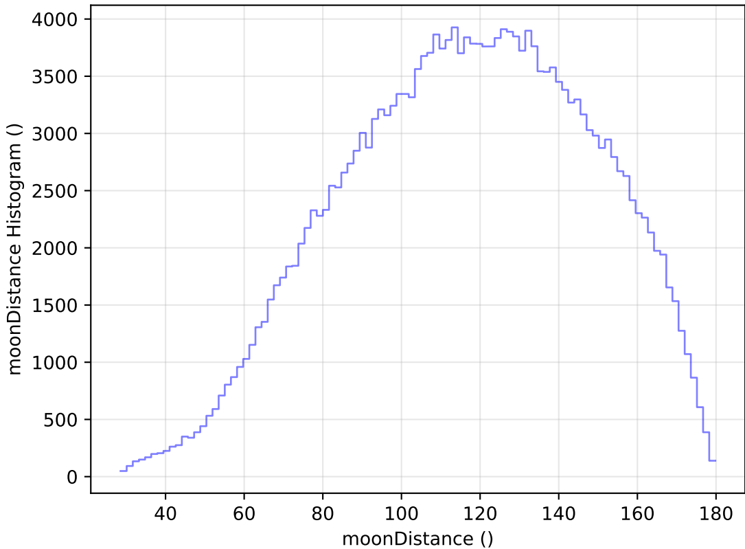
baseline_v2.0_10yrs All sky g band: moonDistance Histogram
